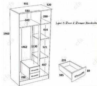
LYNX 3 DOOR 2 DRAWER WARDROBE
